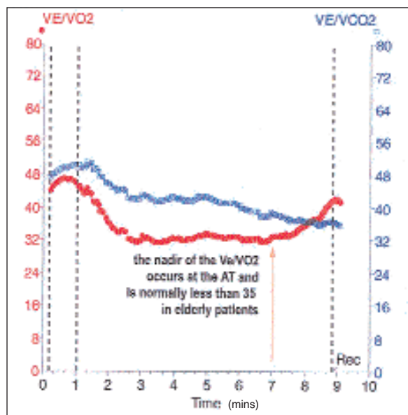
Figure 4. Relationship of the minute volume ( VE ; litre/min) to the oxygen uptake ( VO_2 , red; litre/min) and carbon dioxide output ( VCO_2 , blue; litre/min). These are the ventilatory equivalents. AT = anaerobic threshold; VE/VO_2 = ventilatory equivalent for oxygen; VE/VCO_2 = ventilatory equivalent for carbon dioxide.
